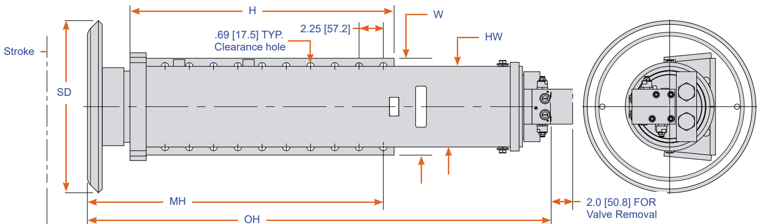
Stabilization Leg – 3 in. (76mm) Bore – Load capacity of 16,000 lb. or 71.2kN
